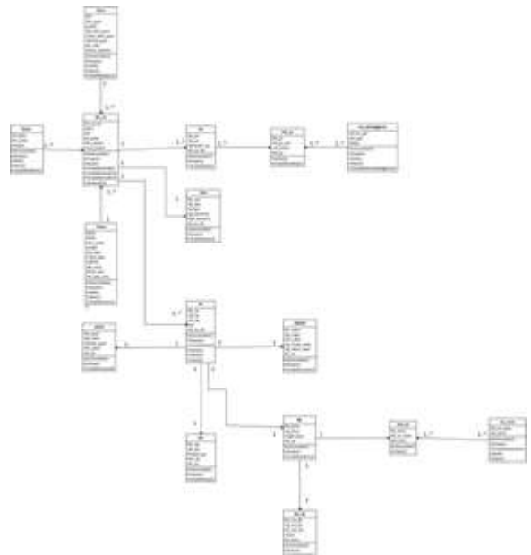
Gambar 10. Class Diagram
