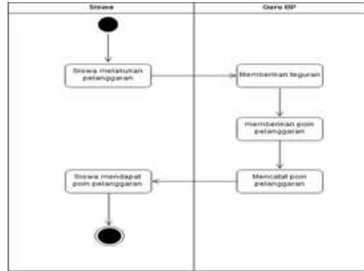
Gambar 2. Activity Diagram Proses Pelanggaran Siswa
